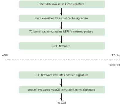
macOS T2 secure boot chain.
